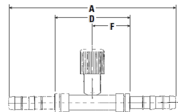
Splicer With High Side R134a Port
