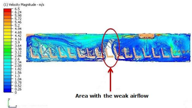
Passenger comfort analysis of bus
