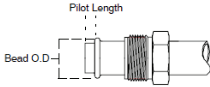
Male O-Ring
