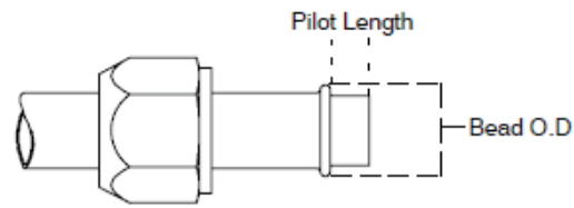
Female O-Ring
