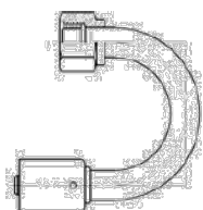
180° Female O-Ring
