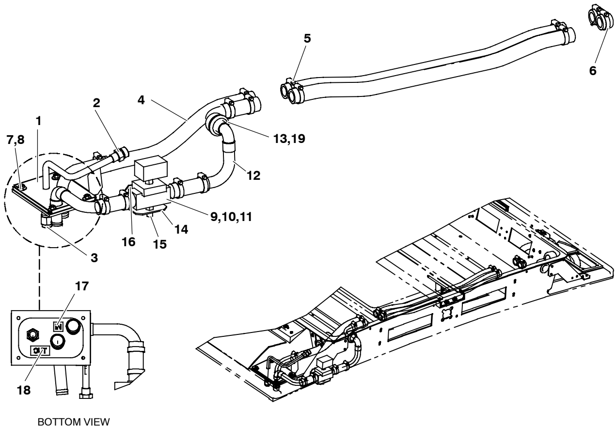
BOTTOM VIEW
