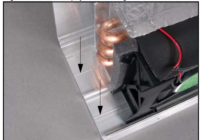
Figure: The notches helps you when drilling the holes
